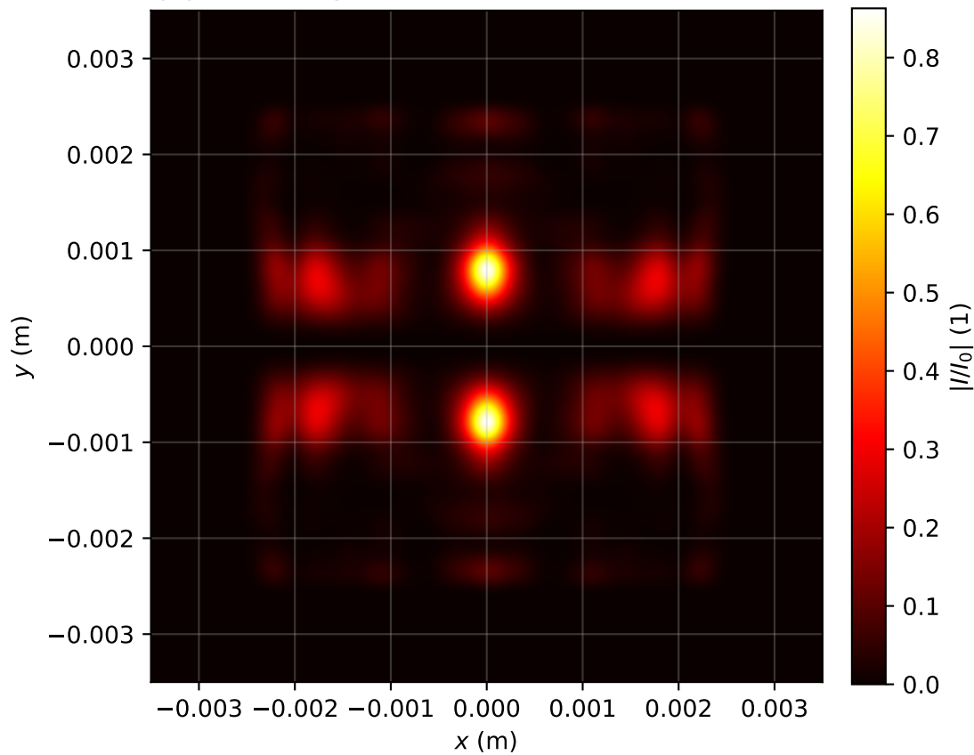
Intensity profile I(x, y, z = 3.742)/I_0 , P_{in}=5.0P_{cr} , artificial time
